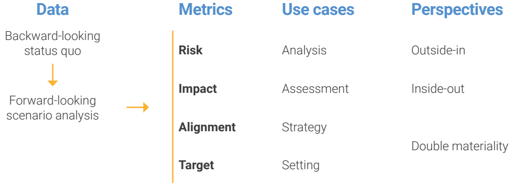
Figure 3: Transition metrics landscape (Julia Bingler, for UNEP FI, 2023)
