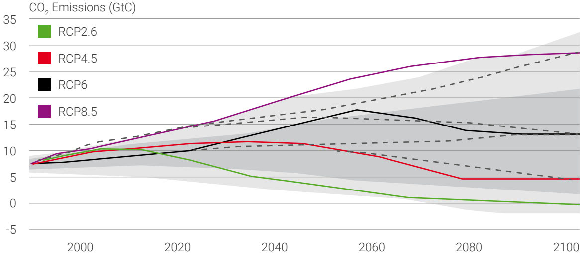
Figure 5: Emissions of carbon dioxide across the RCPs (van Vuuren et. al., 2011).
