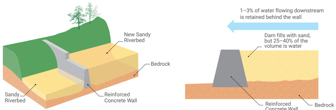
FIGURE 9.4 Sand Dam
