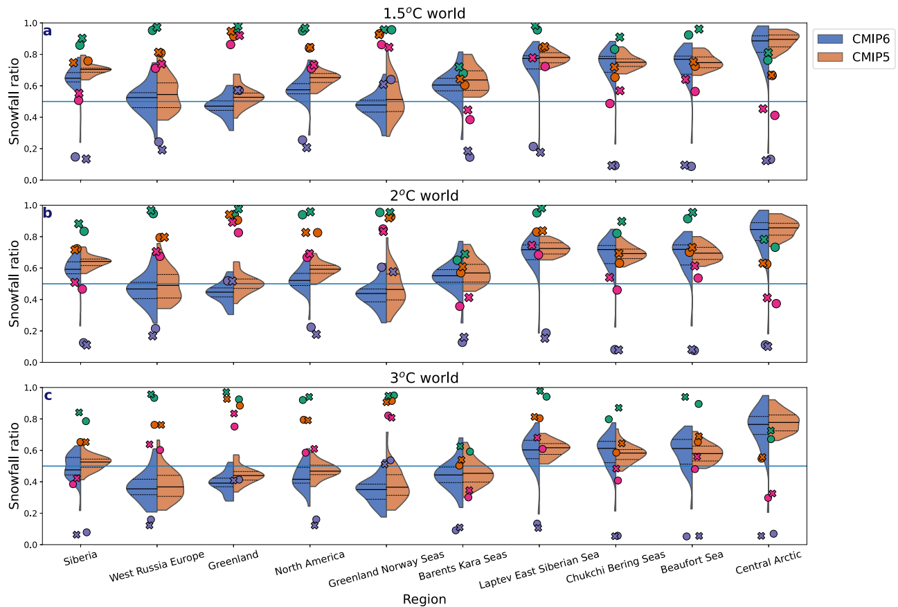
Fig. 10 Snowfall ratio per region in a 1.5 °C, 2 °C and 3 °C global warming scenarios. The snowfall ratio for different regions (identified in Supplementary Fig. 4) across the Arctic following 1.5 °C, 2 °C and 3 °C global warming for CMIP6 (blue) and CMIP5 (orange) with the dashed black lines showing the 25th–75th and the solid black lines showing the multi-model mean. The solid blue line identifies when the snowfall ratio is at 0.5. The circles and x's represent the multi-model ensemble mean snowfall ratio at 1.5 °C, 2 °C and 3 °C for CMIP6 (circles) and CMIP5 (x's) for December–February (green), March–May (orange), June–August (purple) and September–November (pink).
