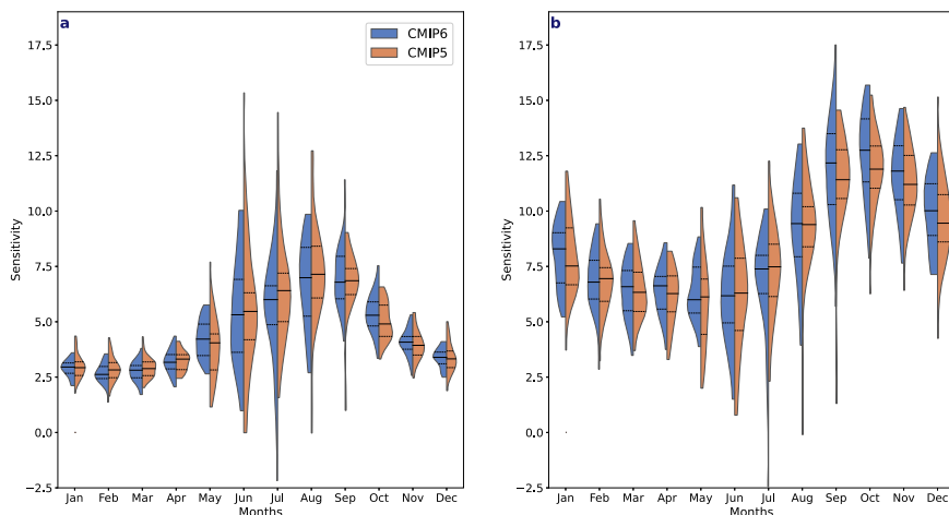
Fig. 4 Sensitivity of precipitation to temperature change throughout the twenty-first century. The percentage change of total precipitation per degree of a Arctic warming and b Global warming by month. The black dashed lines represent the 25th–75th percentile and the black solid lines represent the model mean following the SSP5–8.5/RCP8.5 scenarios for CMIP6 (blue) and CMIP5 (orange).
