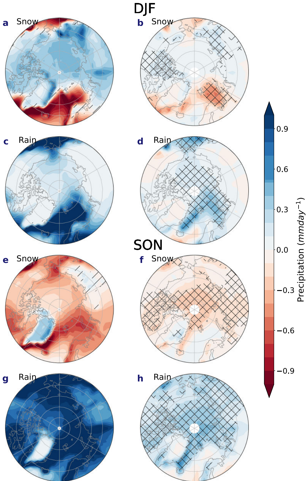
Fig. 3 Snowfall and rainfall changes in CMIP6 and difference between CMIP6 and CMIP5 snowfall and rainfall at the end of the century. The left-hand column shows the changes in a, e snowfall and c, g rainfall at the end of the century in a, c December-February (DJF) and e, g September-November (SON) in CMIP6. Straight line hatching indicates regions where differences are not statistically significant at the 95% confidence level. The right-hand column shows the difference in b, f snowfall and d, h rainfall at the end of the century (2091-2100) relative to the start of the century (2005-2014) between CMIP5 and CMIP6 (CMIP6-CMIP5) for b, d December-February and f, h September-November. Hatching indicates statistical significance at 95% confidence level.
