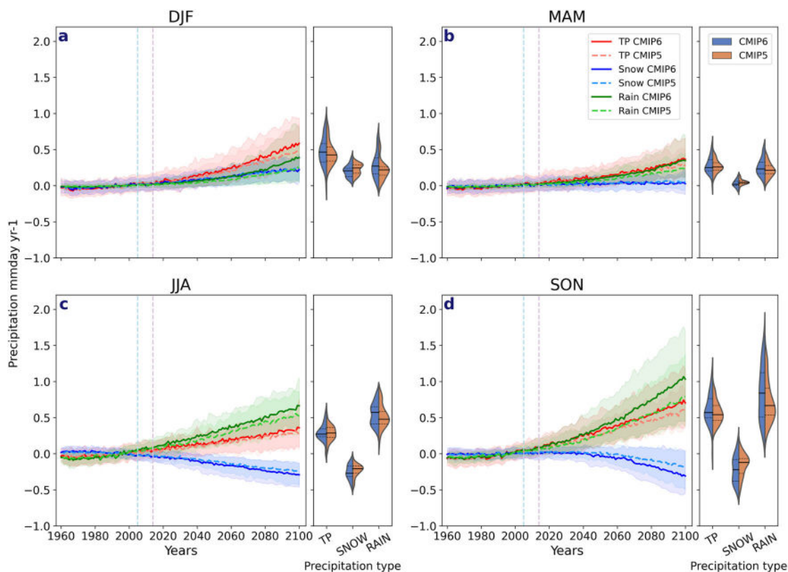
Fig. 2 Time series of total precipitation, snowfall and rainfall anomalies. Changes in total precipitation (TP) (red, orange), snowfall (snow) (blue, light blue) and rainfall (rain) (green, light green) in CMIP6 and CMIP5 are shown relative to the 1981–2009 climatological mean for a December–February (DJF), b March–May (MAM), c June–August (JJA) and d September–November (SON). The light blue vertical dashed line denotes when the historical period for CMIP5 ends and the light purple vertical dashed line denotes when the historical period of CMIP6 ends and thereafter the RCP8.5 and SSP5–8.5 climate scenarios for CMIP5 and CMIP6 are used. The shading around each line highlights the spread based upon the lower 5th and 95th percentiles among the model members. The violin plots represent the model spread from 2090 to 2100 for each total precipitation (TP), snowfall (snow) and rainfall (rain) with the dashed black lines representing the 25th and 75th percentiles, and the black vertical line representing the mean of all models.
