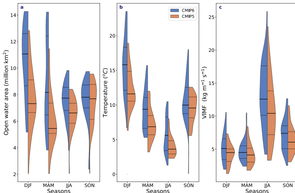
Fig. 6 End-of-century changes in sea-ice concentration, temperature and vertically integrated moisture flux. The end-of-century (2090–2100) changes relative to the start of the century (2005–2014) in all seasons in a open water area (million squared km), b temperature (°C) and c vertically integrated moisture flux (VIMF) at 70°N ( \text{kg m}^{-1} \text{s}^{-1} ) for CMIP6 (blue) and CMIP5 (orange), where the colours represent the kernel distribution of all models. The solid black lines represent the multi-model ensemble means for both experiments and the dashed black lines denote the 25th and 75th percentile in each experiment.
