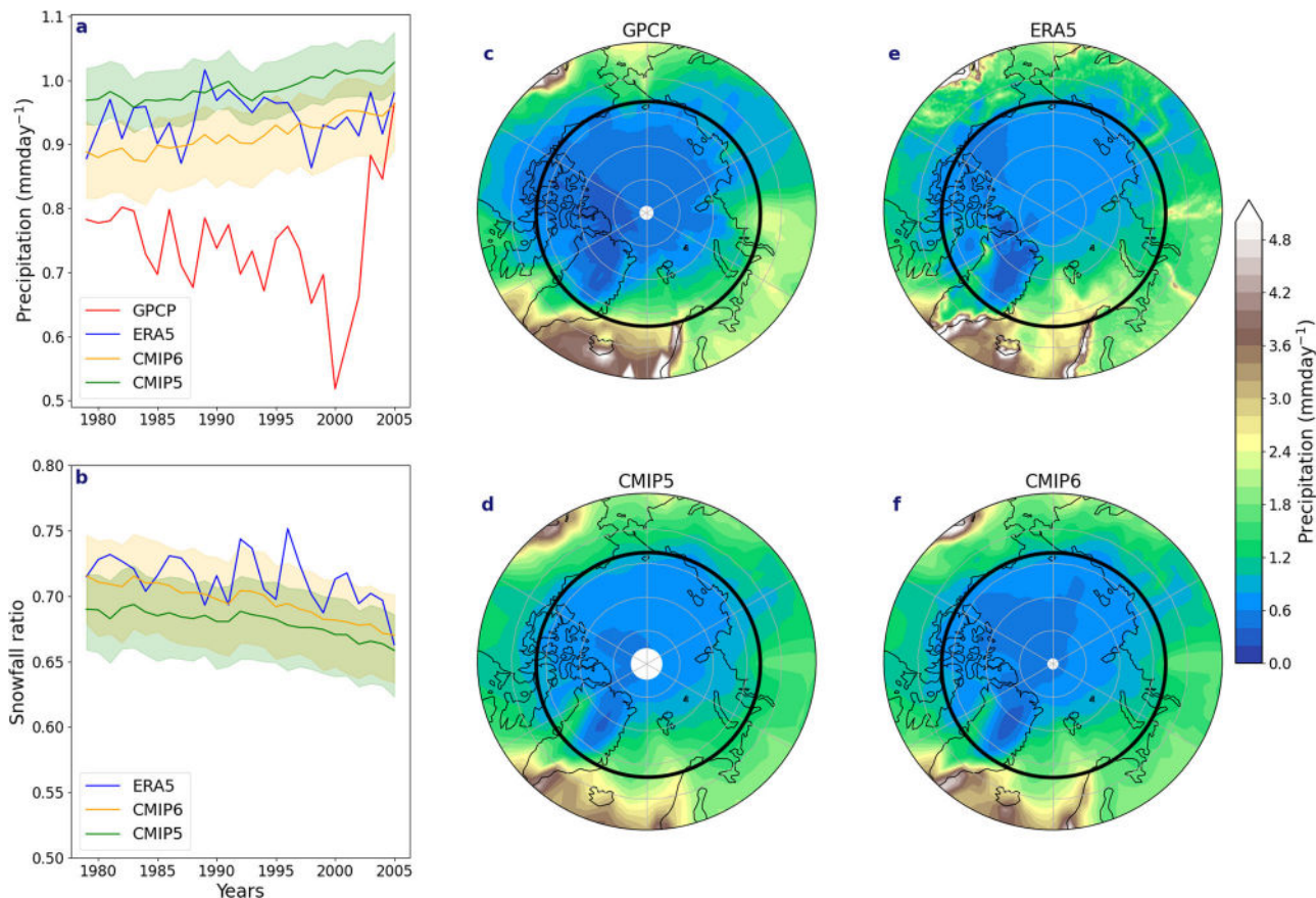
Fig. 1 Time series of precipitation, and snowfall ratio and spatial climatology of total precipitation. a Annual precipitation means over the Arctic (70°N–90°N) from 1979 to 2005, covering the satellite era and the start of the GPCP record concluding with the end of the historical period for GPCP, ERA5, CMIP5 and CMIP6. b Annual snowfall ratio (snowfall/total precipitation) over the Arctic for the same observational record of 1979–2005 for ERA5, CMIP6 and CMIP5. The shading in both represents the 5th to 95th percentile spread in the models. Climatological precipitation for the same record over the Arctic for c GPCP, d CMIP5, e ERA5 and f CMIP6. The Arctic region for all time series analyses is taken as the area poleward of 70°N, shown as the dark circle in c–f .
