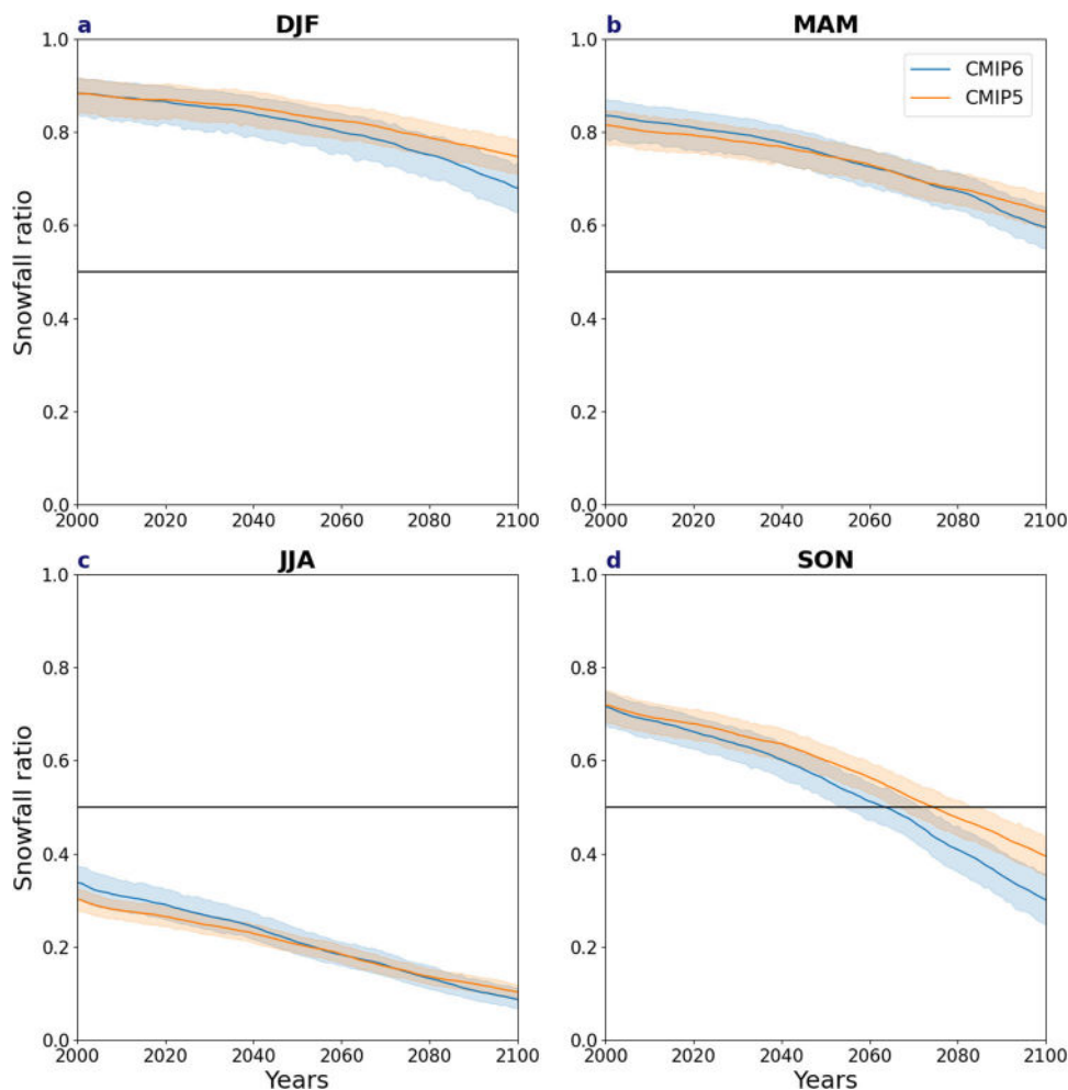
Fig. 9 Time evolution of the snowfall ratio. The snowfall ratio over time. The horizontal lines denote the transition from a snow- to rain-dominated precipitation at (0.5) for CMIP6 (blue) and CMIP5 (orange) for a December–February (DJF), b March–May (MAM), c June–August (JJA), d September–November (SON). The shading indicates 5th–95th model spread for each and all data are averaged as a 10-year rolling mean.
