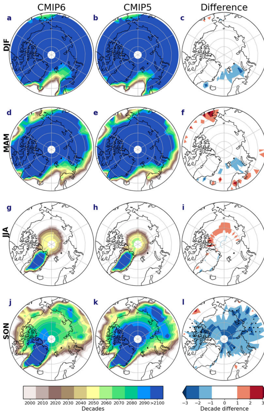
Fig. 8 Decade of transition between snow-dominated precipitation to rainfall-dominated precipitation and their differences. The decade of transition from a snow-dominated precipitation regime to a rain-dominated regime for CMIP6 [first column] and CMIP5 [second column] multi-model ensemble means, taken as when annual snowfall relative to annual precipitation falls below 50% and their differences [third column] for a-c December–February (DJF), d-f March–May (MAM), g-i June–August (JJA) and j-l September–November (SON). Areas that do not transition by 2100 are shaded in blue. Areas shaded in white in the first two columns are rain-dominated before the year 2000.
