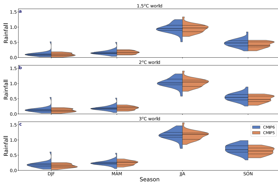
Fig. 7 Arctic rainfall changes per season relative to global warming scenarios. The Arctic rainfall change in \text{mm day}^{-1} with respect to 1.5 °C, 2 °C and 3 °C global warming for CMIP6 (blue) and CMIP5 (orange) in December–February (DJF), March–May (MAM), June–August (JJA) and September–November (SON). Dashed black lines show the 25–75th percentiles and the solid black lines show the multi-model mean.
