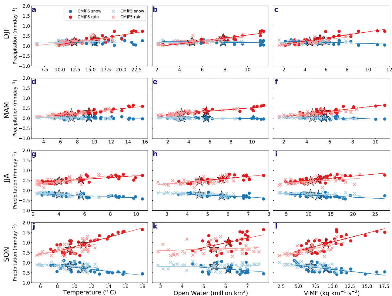
Fig. 5 Model-dependent end-of-century changes in snowfall and rainfall for SSP5–8.5/RCP8.5 forcing. Inter-model dependence of snowfall and rainfall to a, d, g, j surface air temperature, b, e, h, k Open water and c, f, i, l vertically integrated moisture flux (VIMF) changes at the end of the century relative to the start of the century for a–c December–February (DJF), d–f March–May (MAM), g–i June–August (JJA), j–l September–November (SON). Each dot represents a model from CMIP6 and each \times represents a model from CMIP5. The stars represent the multi-model means for either CMIP6 and CMIP5 snowfall/rainfall in the same colours as their representative individual members. The line of best fit is calculated using a 1D polynomial.
