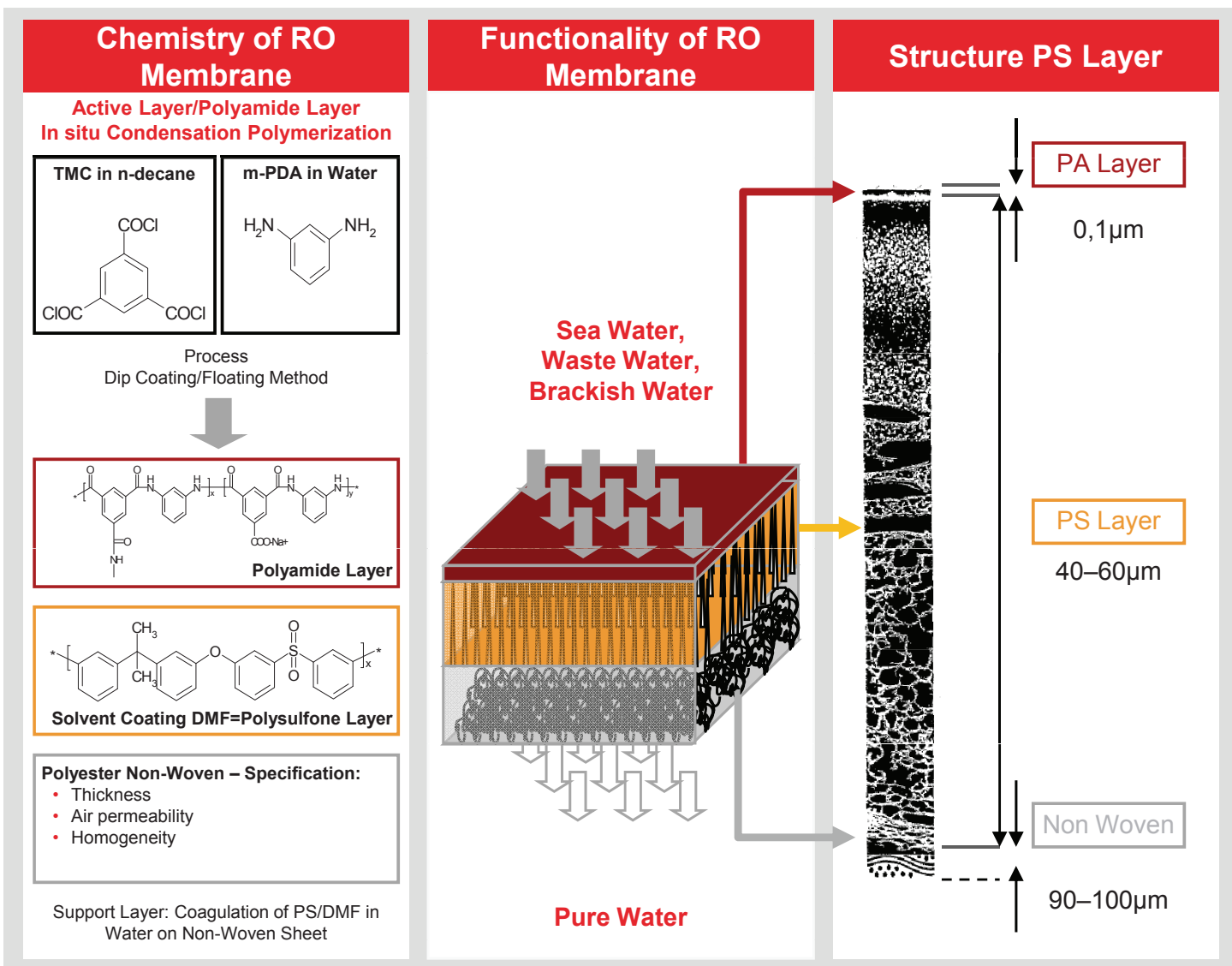
Figure 1: Structure of a thin film composite membrane.
