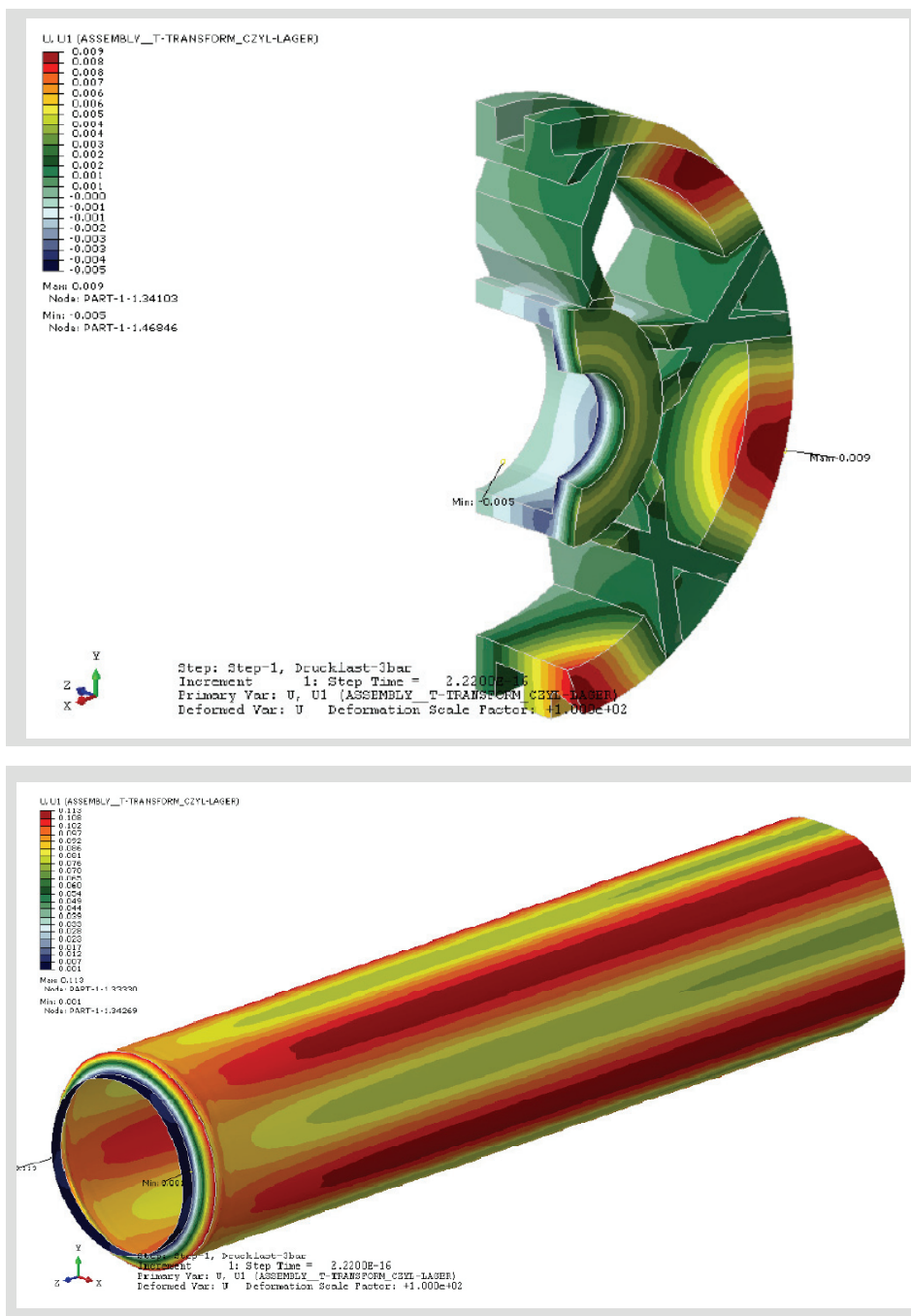
Figure 2: Stress test on the anti telescoping device (ATD) and permeate tube.
